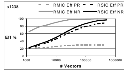
Figure 4: Comparison of RSIC and RMIC sequence efficiencies for circuit s1238
