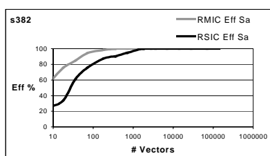
Figure 5: Comparison between stuck-at fault coverage of RSIC and RMIC - circuit s382
