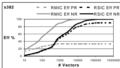
Figure 2: Efficiency comparison of RMIC and RSIC sequences
