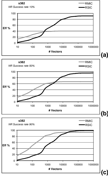
Figure 3: Comparison of weighted efficiencies of RMIC and RSIC sequences for various values of S_{NR} : (a) 10%, (b) 50%, (c) 90%.
